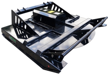
72"Brush&Sapling Mower
